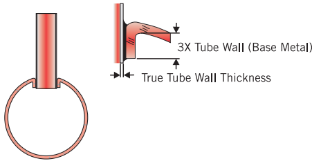
Figure 12 - Cu Tubes to Cu Header Joint
