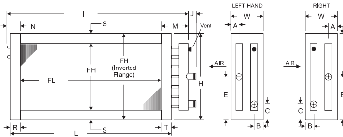
Figure 10 - SS, SH Dimension Info
