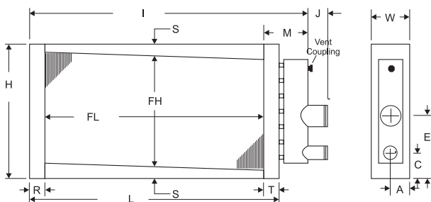
Figure 2 - JA, GA Dimension Info
