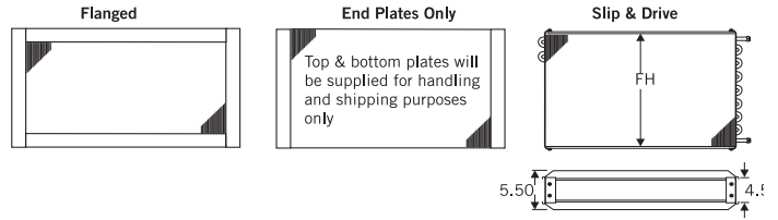
Figure 13 - Case Styles (continued)
