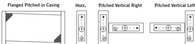
Figure 13 - Case Styles
