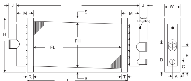
Figure 6 - RA, TA Dimension Info
