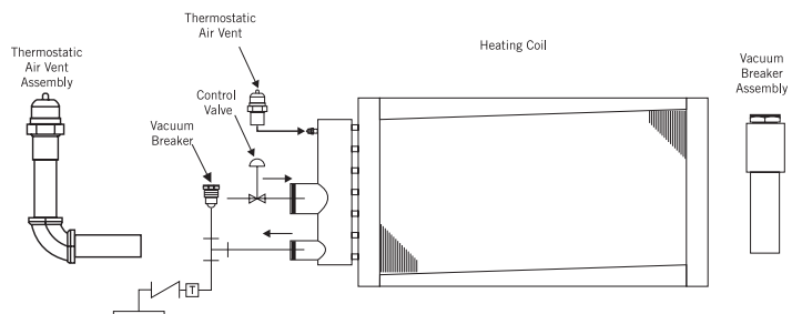
Figure 14 - Vacuum Breaker Assembly
