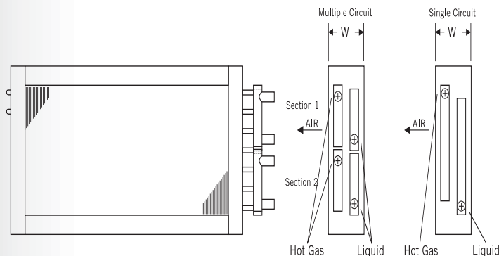
Figure 1 - Condenser Coils
