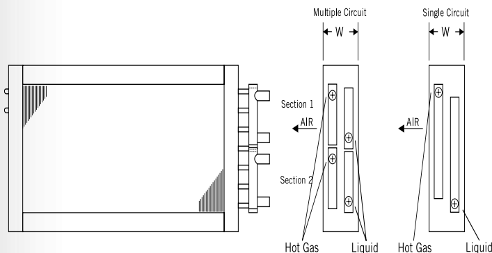
Figure 1 - Condenser Coils
