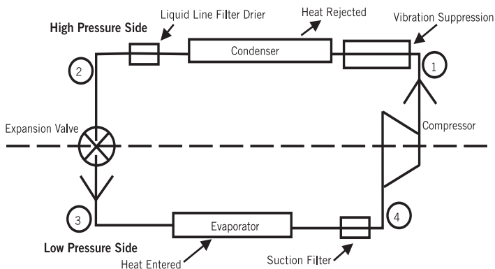
Figure 2 - General Plumbing
