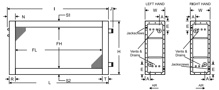
Figure 17 - Cleanable Supply End - Opposite End Connections
