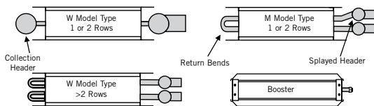
Figure 1 - Standard Coil Types
