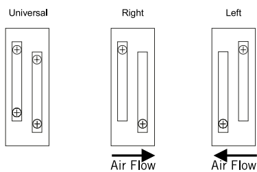
Figure 18 - Connection Location
