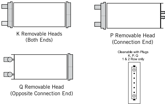
Figure 7 - Cleanable Coil Types
