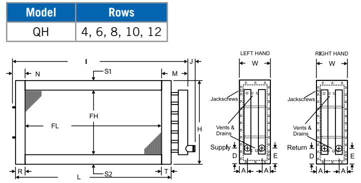
Figure 15 - Cleanable Opposite Supply End - Same End Connection - Half Serp
