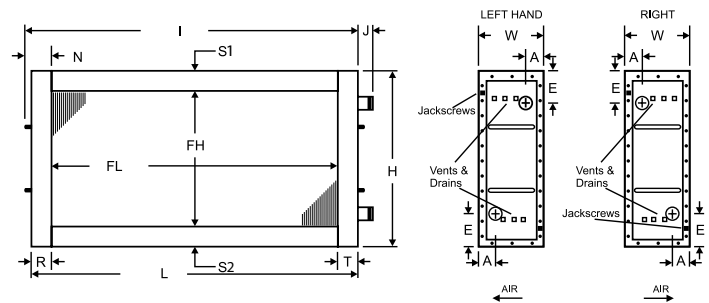
Figure 11 - Cleanable Both Ends - Opposite End Connections
