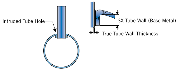
Figure 19 - Brazed Joint
