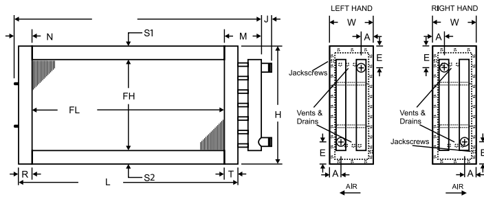
Figure 14 - Cleanable Opposite Supply End - Opposite End Connections
