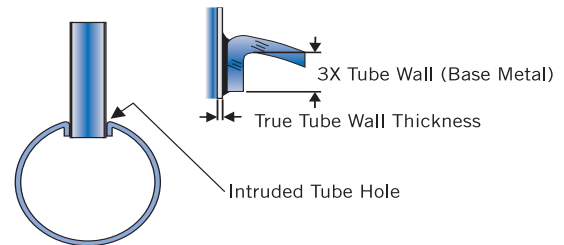
Figure 7 - Brazed Joint
