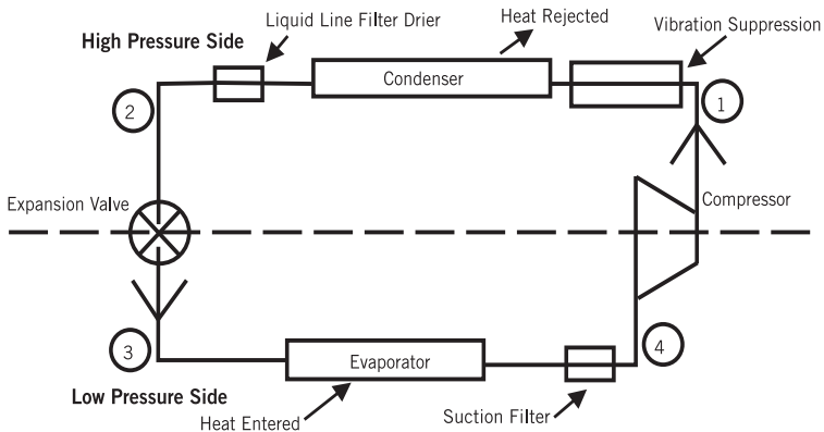
Diagram 1 - Vapor Compression Cycle
